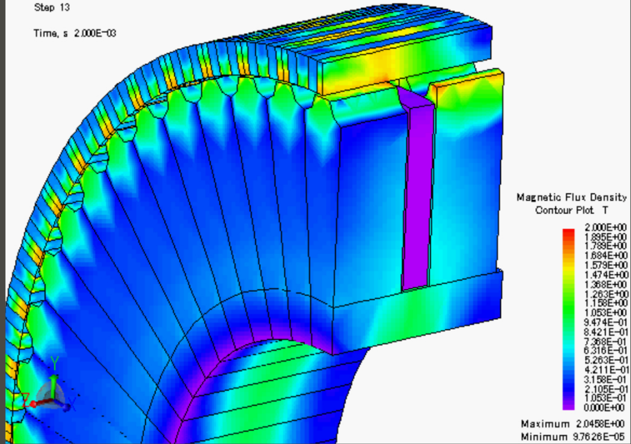
Finite element analysis results showing the magnetic flux density of a generic transverse flux motor.
